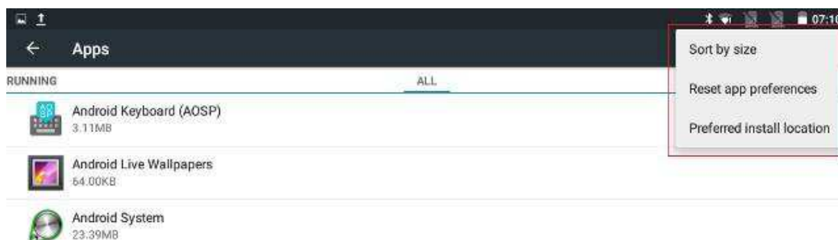
FIGURE 5.34. APPS MENU
