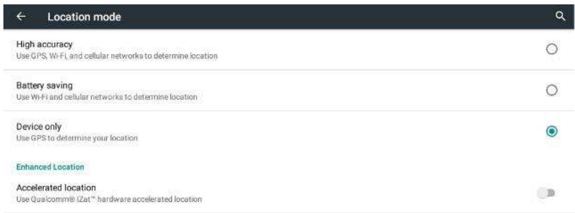
FIGURE 5.37. LOCATION MODE
